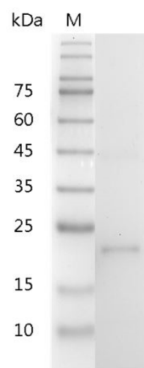
SDS-PAGE analysis of recombinant mouse IL-12 p35
